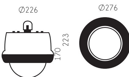
Moon diffuser
