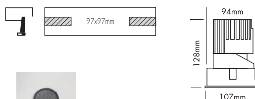
Antiverblindings grid
