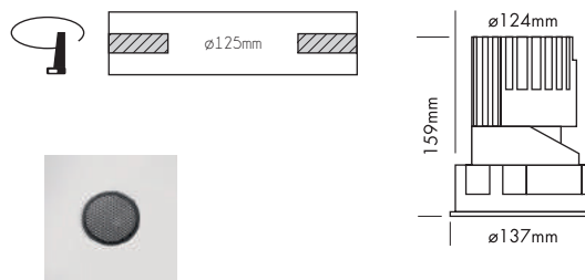
Antiverblindings grid
