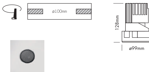
Antiverblindings grid
