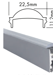
LENS COVER 45°
