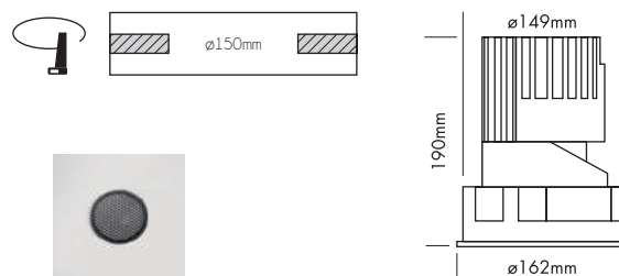
Antiverblindings grid
