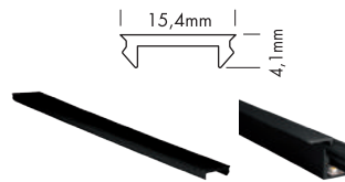
Plastic cover S-Line flat black
